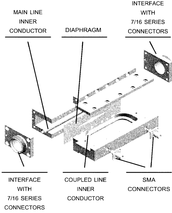
Fig. 2. Scheme of the realized coupler.
