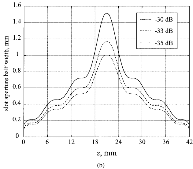
Fig. 3. (a) Target coupling factor \mathcal{K}(z) and (b) designed aperture half-width s^{\text{opt}}(z) for the three realized couplers.
